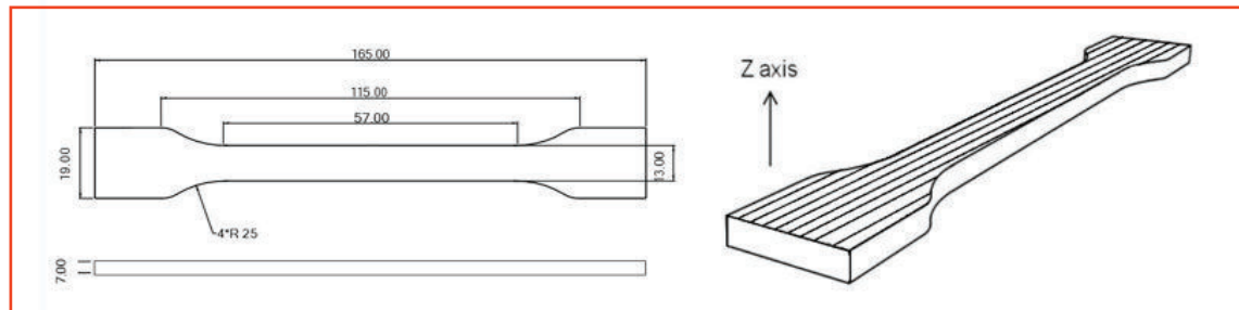
Figure 1. Tensile testing (axis 1) specimen
