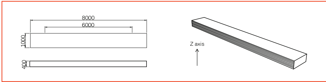
Fig 10. Flexural testing specimen
